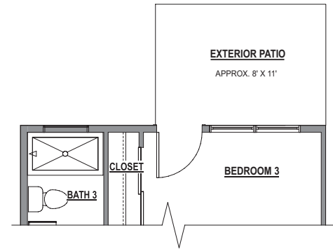
Plan A - Second Level Patio Option
