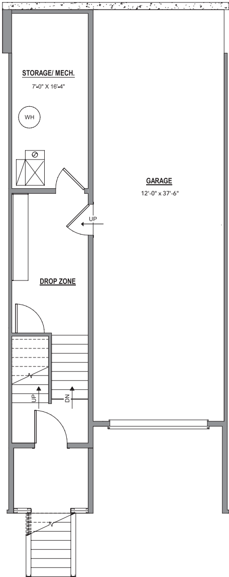
Plan A - Main Level
